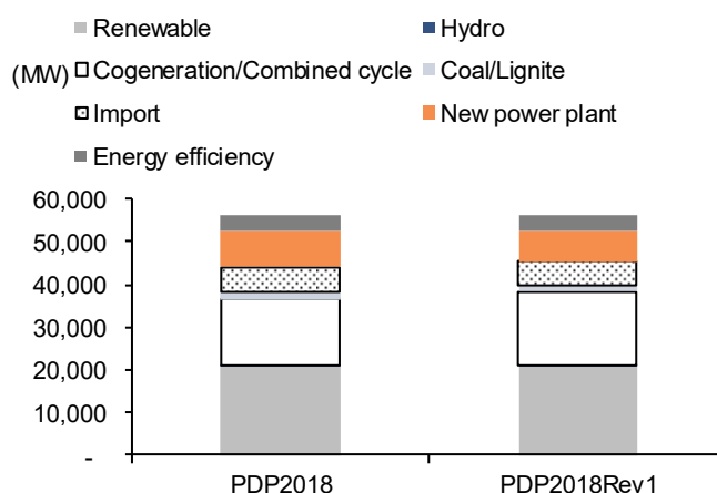
Exhibit 2: Power capacity breakdown under PDP 2018
