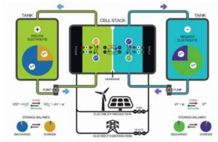
Exhibit 1: Vanadium redox battery
