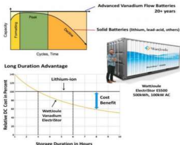
Exhibit 5: VRFB's lifecycle and rechargeable lifetime is longer than lithium-ion batteries
