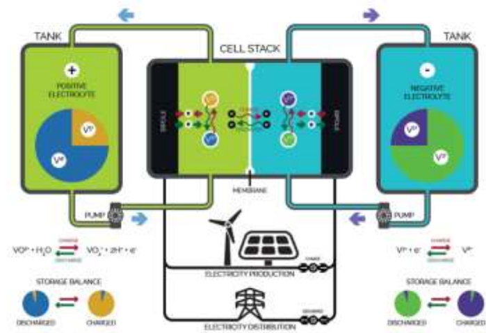
Exhibit 1: VRFB's two components – cell stacks and external electrolytes
