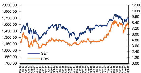
SET Index
