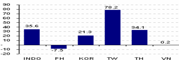
US$mnn Foreign Fund Flow by Country (06 Feb 2017)
